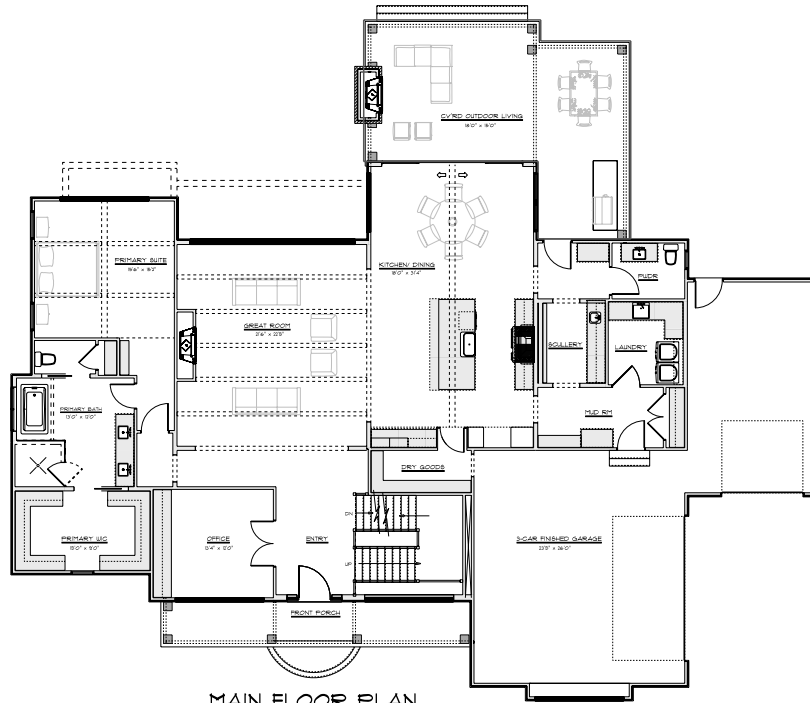
MAIN FLOOR PLAN 2,795 SF
